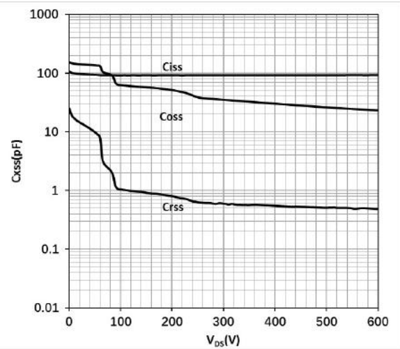
Figure 19 Typ. capacitances
